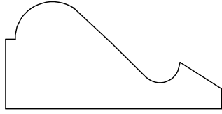
BASE CAP 21385 11/16" X 1 3/8" (SIMILAR TO WM 163)
