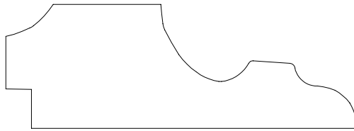
BASE CAP 22633 29/32 " X 2\ 19/32 " ( 9/32 " KNOTCH)
