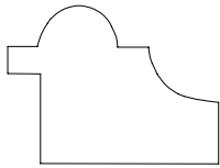
CUSTOM BASE CAP 210016 3/4" X 1" (7/16" KNOTCH)
