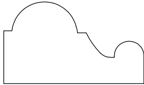
BASE CAP 21386 13/16" X 1 3/8"
