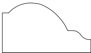
BASE CAP 21254 11/16" X 1 1/4"
