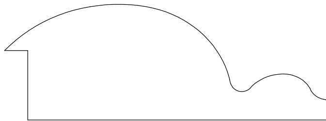
BASE CAP 235017 1 1/4" X 3 1/2" 1/4" X 3/4" THROAT
