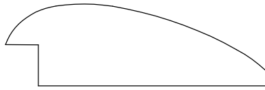
BASE CAP 22004 5/8" X 2" 1/4" X 5/16" THROAT
