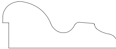
BASE CAP 22007 13/16" X 2" 1/8" X 1/2" THROAT
