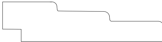
BASE CAP 232512 13/16" X 3 1/4"
