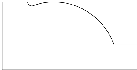
BASE CAP 21759 7/8" X 1 3/4"
